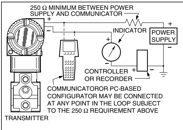
Figure 19. HART 4 to 20 mA Topology
