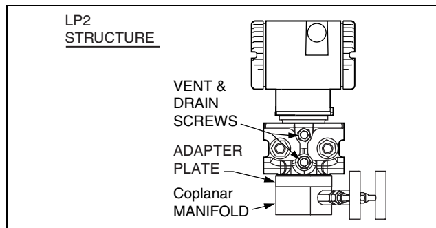
Figure 14. Adapter Mount to Existing Coplanar Manifold
