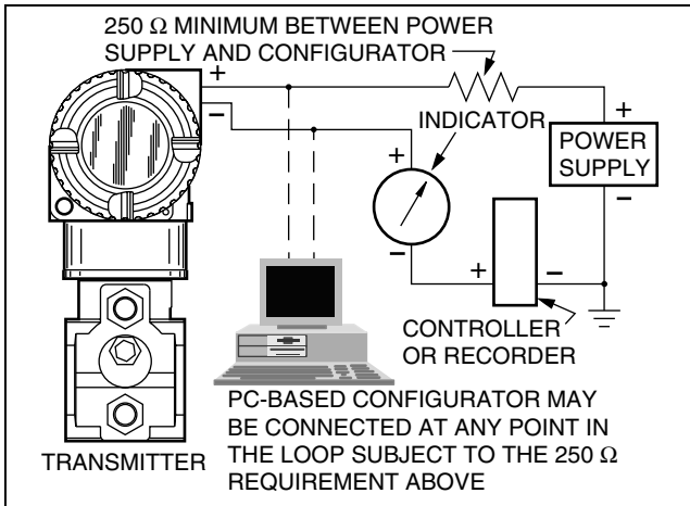
Figure 18. FoxCom 4 to 20 mA Topology
