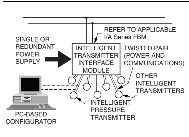
Figure 21. FoxCom Digital Topology
