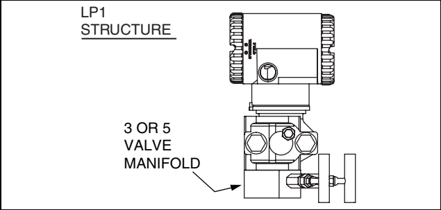
Figure 7. LP1 Shown Directly Mounted to Manifold
