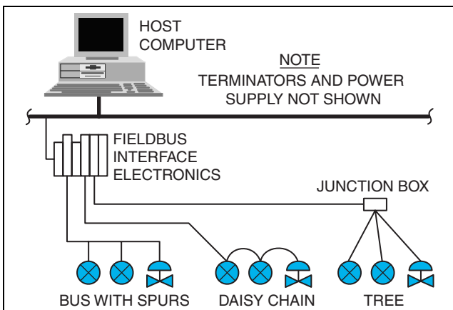
Figure 20. Fieldbus Miscellaneous Topologies
