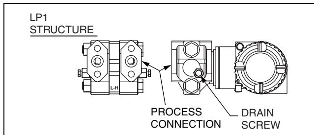
Figure 11. Horizontal Mounting with Drain Screw
