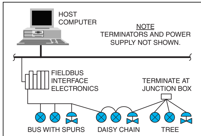
Figure 23. Fieldbus with Mixed Topologies
