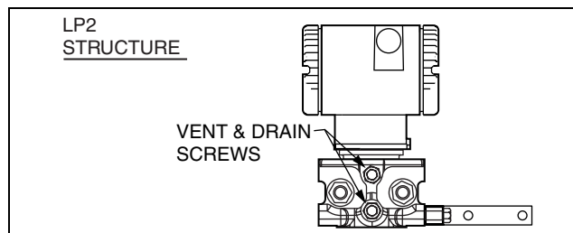
Figure 13. Shown on Coplanar Bracket
