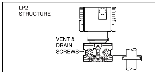
Figure 12. Shown on Foxboro Universal Bracket
