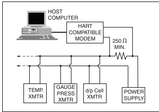
Figure 22. HART Multidrop Topology
