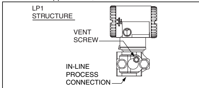
Figure 9. Upright Mounting
